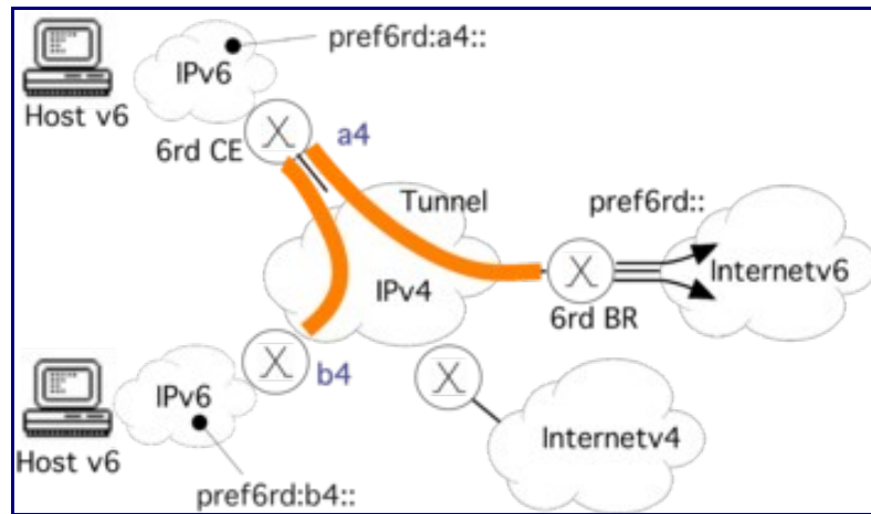
Figure 12: Architecture de 6rd.
